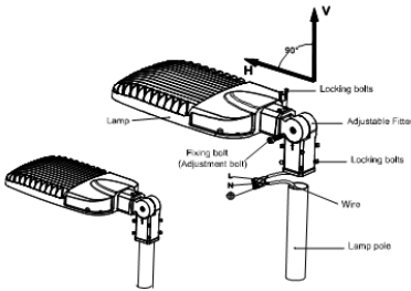
BRACKET A Slip Fitter Mount (adjust from -90^{\circ} ~ +90^{\circ} )
