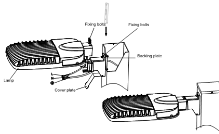
BRACKET D Fixed Square Pole Mount
