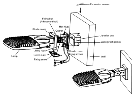
BRACKET F Wall mount (adjust from -90^{\circ} ~ +90^{\circ} )
