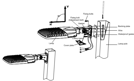
BRACKET D Fixed Square Pole Mount
