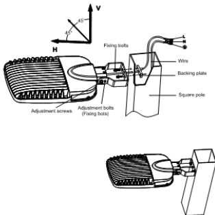
BRACKET E Trunnion (adjust from -90^{\circ} ~ +90^{\circ} )
